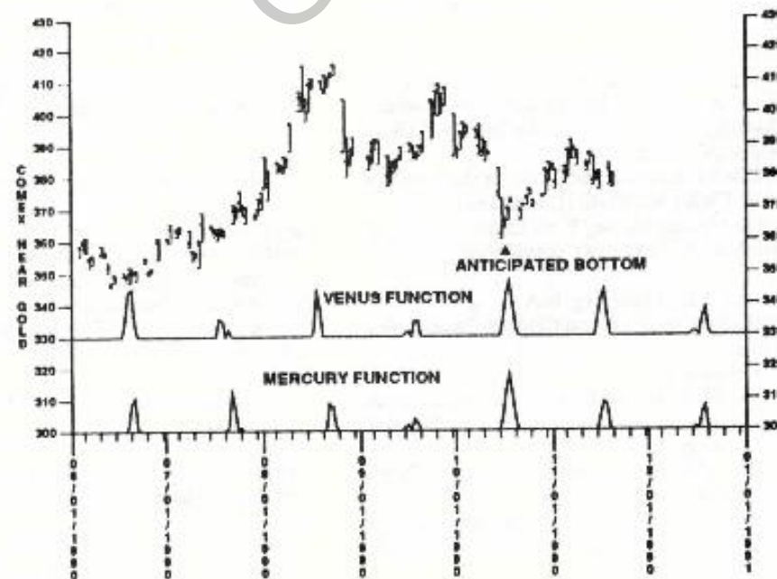
FIG. 6. Using the two lunar chaos functions.
